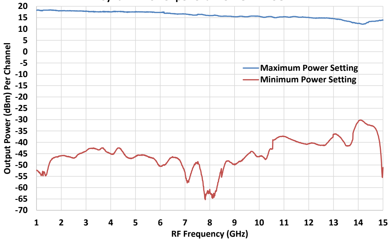
SynthHD Power per Channel 1GHz - 15GHz
