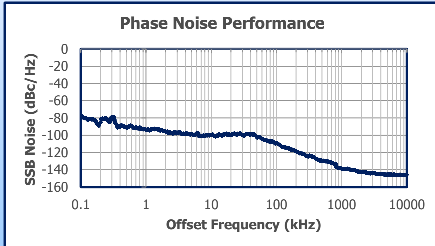
Phase Noise @ 16.3 GHz, 10MHz Ref
